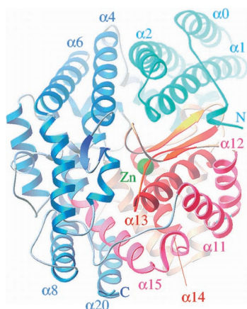
Figure 6. Ribbon structure of Oligoendopeptidase F. The protein has neurolysin topology with a mainly \alpha -helical scaffold. The central groove divides the protein into two “subdomains” (shown in cyan and red). One \text{Zn}^{2+} ion (shown as a small, green sphere) is bound at the active site. The helix \alpha 13 contains the HEXXH zinc-binding motif with its two zinc-coordinating histidine residues (His 356 and His 360). Additional coordination is provided by Glu 384 on helix \alpha 14 . The \alpha -helix numbering from the PDB 1O86 structure [29] was used.
