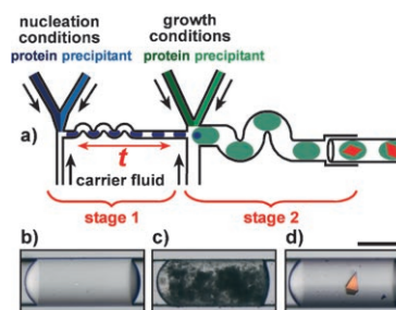
Figure 2. a) The process of microfluidic seeding. In stage 1 of the device, solutions at concentrations that promote nucleation are combined. After a delay ( t = 3–15 s, depending on the flow rate), seed crystals formed in stage 1 are merged into stage 2 of the device, where solutions that promote crystal growth are combined. b–d) Microphotographs of typical plugs containing thaumatin: b) at low supersaturation (growth conditions) no nucleation occurs and no crystals form; c) at high supersaturation (nucleation conditions) precipitation occurs; d) a single thaumatin crystal was nucleated in stage 1 and grown in stage 2. Scale bar: 200 \mu\text{m} .
