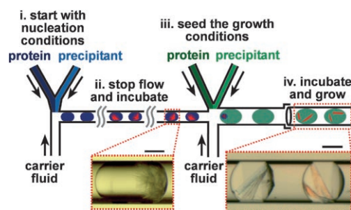
Figure 4. Separating the stages of nucleation and growth in the crystallization of "SARS protein" yields single crystals. i) Protein and precipitant solutions of high concentration are combined to form plugs. ii) The flow is stopped, and the plugs are incubated to generate seed crystals (left microphotograph: a typical "SARS protein" crystal grown in solutions of high supersaturation in which excess nucleation leads to clustered microcrystals). iii) Protein and precipitant solutions of lower concentration are combined to form plugs containing solutions at a lower degree of supersaturation that lead to crystal growth. Each plug containing seed crystals seeds multiple growth plugs. iv) Growth plugs that contain seed crystals are flowed into a glass capillary and incubated (right microphotograph: two typical plugs of low supersaturation that have been seeded with "SARS protein" microcrystals). Scale bars: 100 µm.
